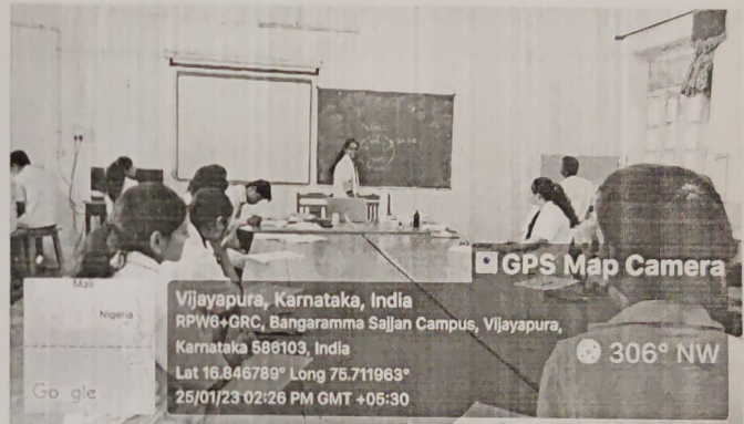
Vijayalaxmi - Plasmid
